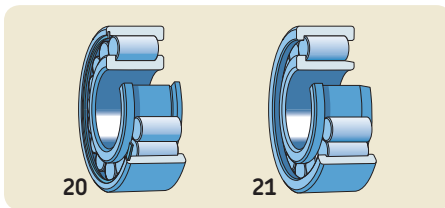
Full complement cylindrical roller bearings single row NCF design (20) NJG design (21)
