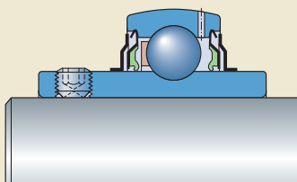
a) Grub (set) screw locking
