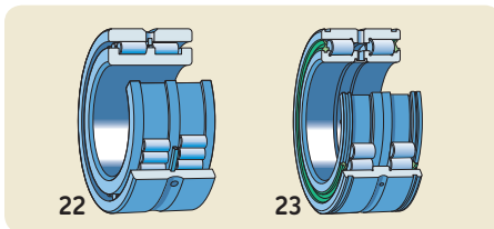
double row with integral flanges on the inner ring (22) with integral flanges on the inner and outer rings with contact seals (23)
