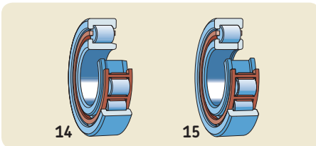
single row NJ design (14) with angle ring NUP design (15)
